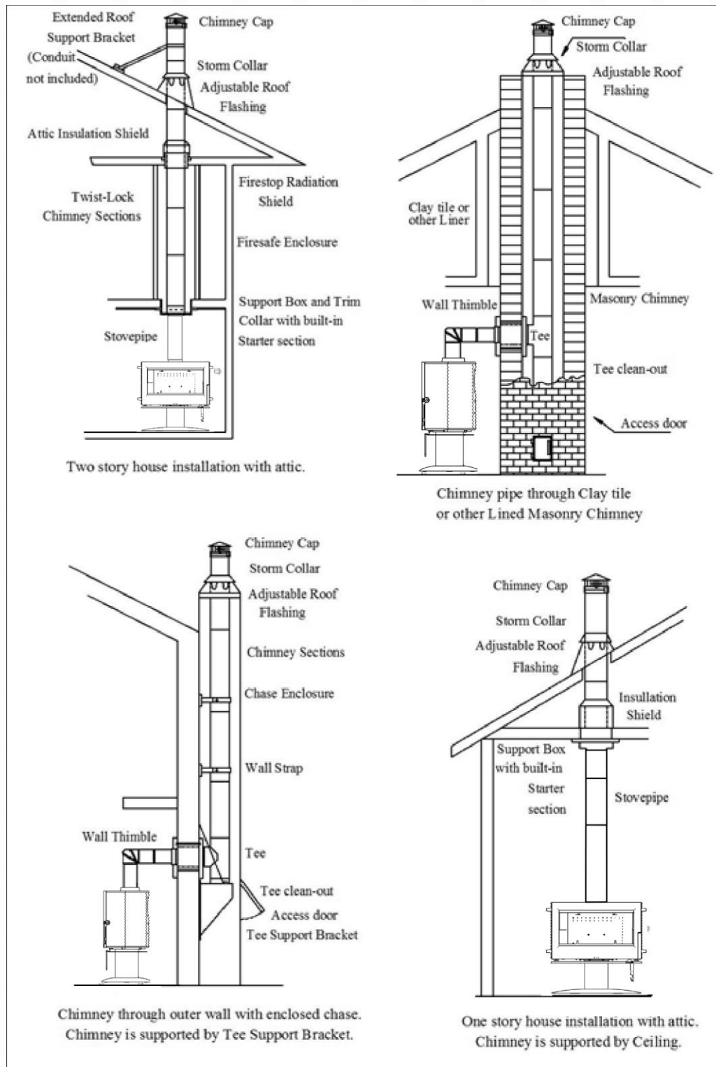
Figure 9 – Typical Chimney Configurations
