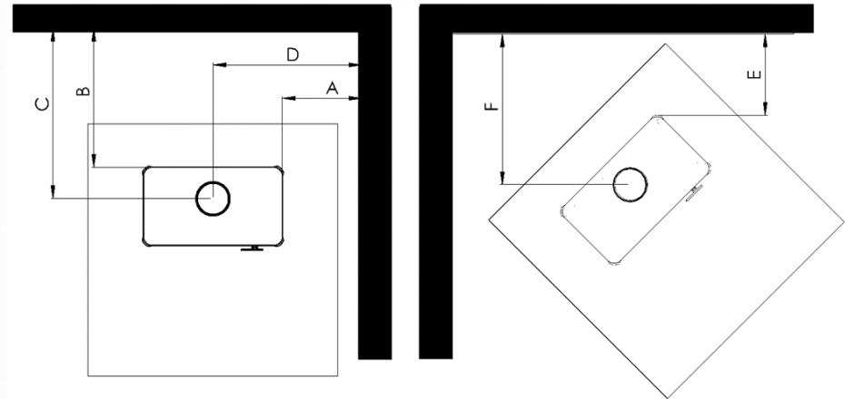
Figure 4 – Clearance to Combustibles
