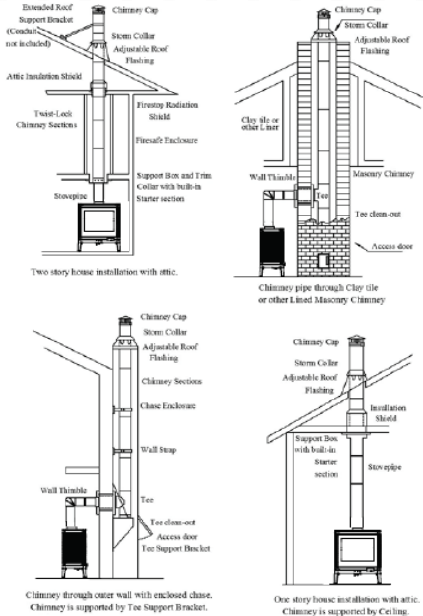
Figure 9 – Typical Chimney Configurations
