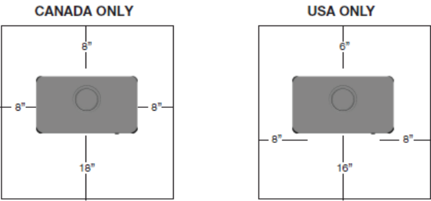
Figure 3 – Hearth Dimensions
