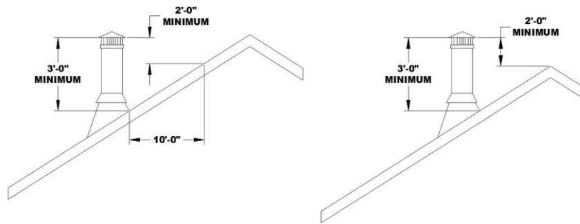
Figure 8 – Chimney Height Requirements
